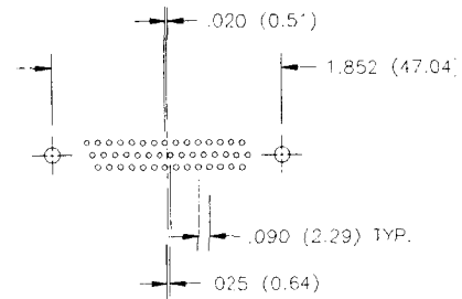
44 Position - Shell Size B
