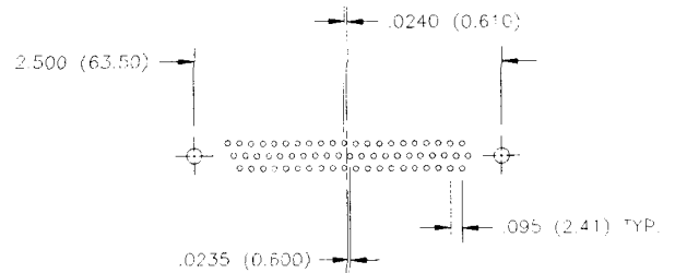
62 Position - Shell Size C
