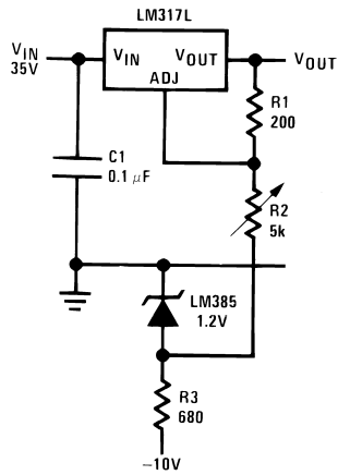
0V–30V Regulator
