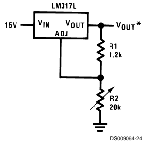
1.2V–12V Regulator with Minimum Program Current
